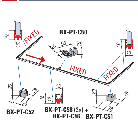
A SET 3 L = 2200 / L = 3000 mm
