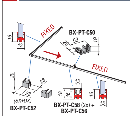
A SET 4 L = 2200 / L = 3000 mm
